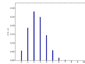
FIGURE 1 – Loi \mathcal{B}(10, 1/4)
